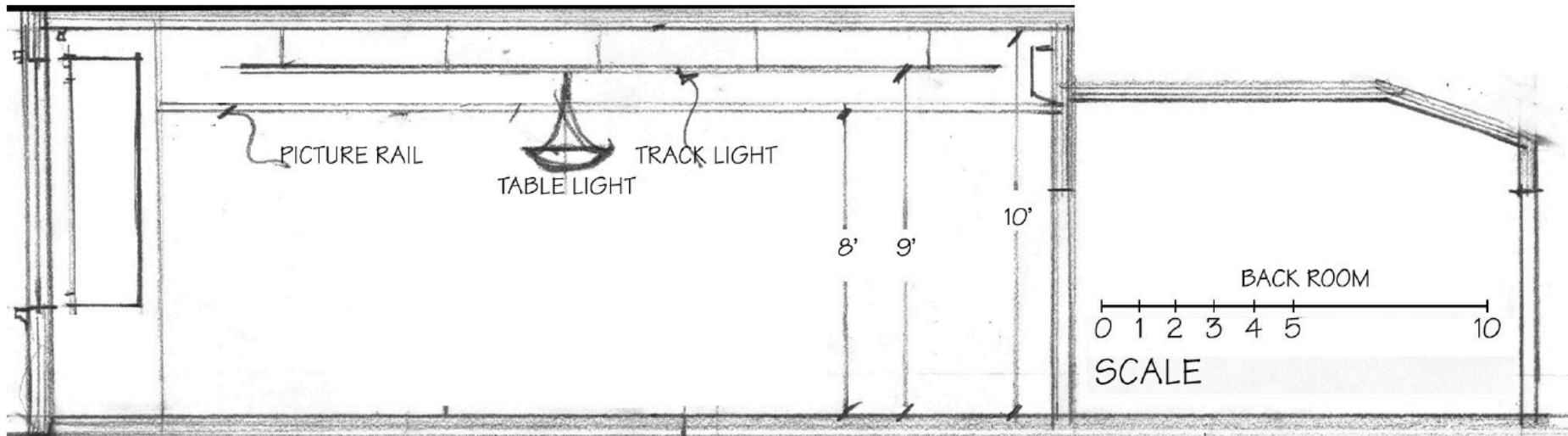
WALL ELEVATION
