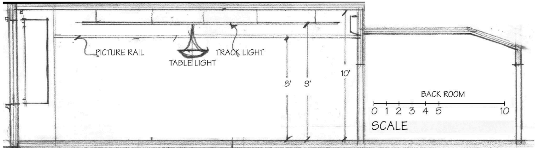
WALL ELEVATION
